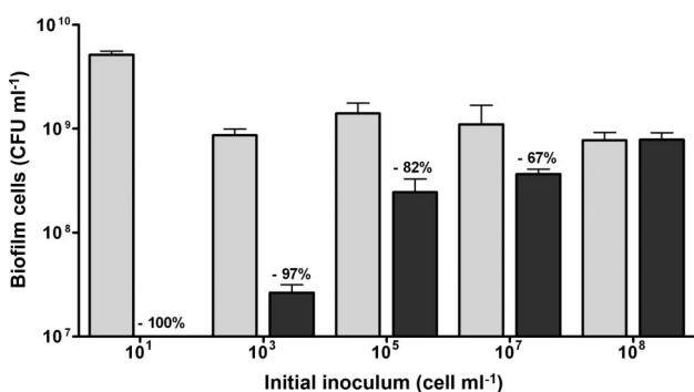
Figure 1. Prevention of biofilm formation using SAW. Catheters were challenged with different P. aeruginosa inoculum concentrations with and without SAW. Presented are CFU ml -1 obtained following incubation for 3 days in catheters in the presence (black) or absence (grey) of SAW. The bars are an average of at least three independent experiments; the error bars represent SD. The percentages above the bars represent the effectiveness of prevention of biofilm formation.
